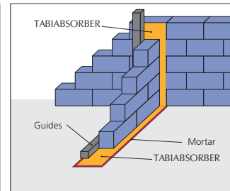
The Tabiabsorber can be cutted in bands
