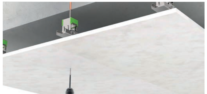
12.- Position plasterboards in place.
